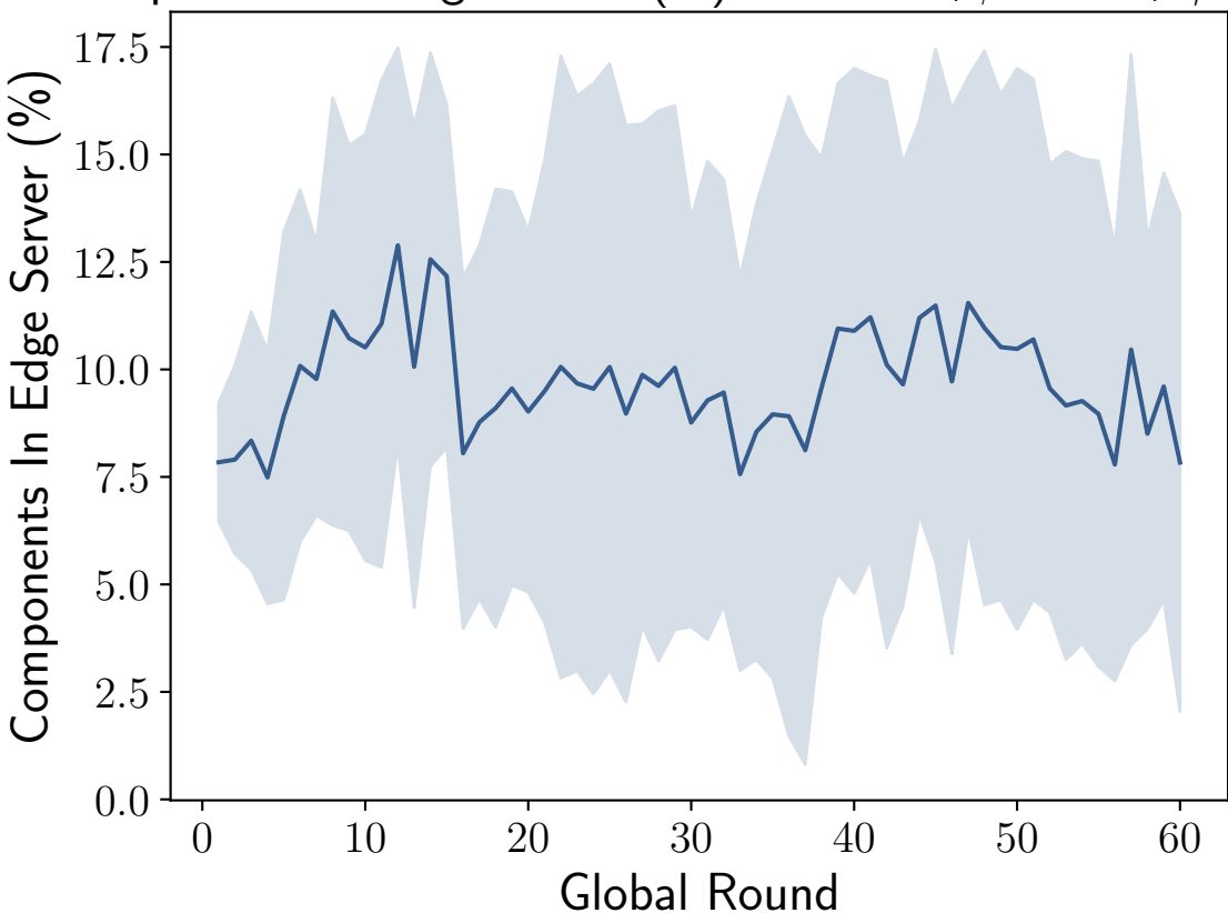
Components In Edge Server (%) - \alpha = 1.0 , \beta = 0.0 , \gamma = 0.0
